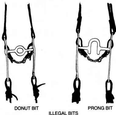
ILLEGAL BITS
